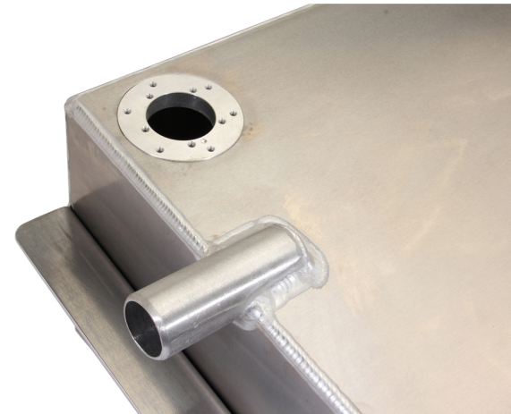
6372AGT-20S CLOSEUP.jpg
